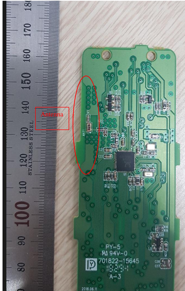
Antenna View
