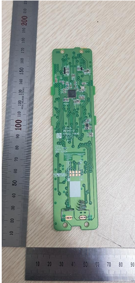
PCB – Front View
