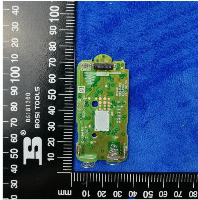
PCB – Rear View 2
