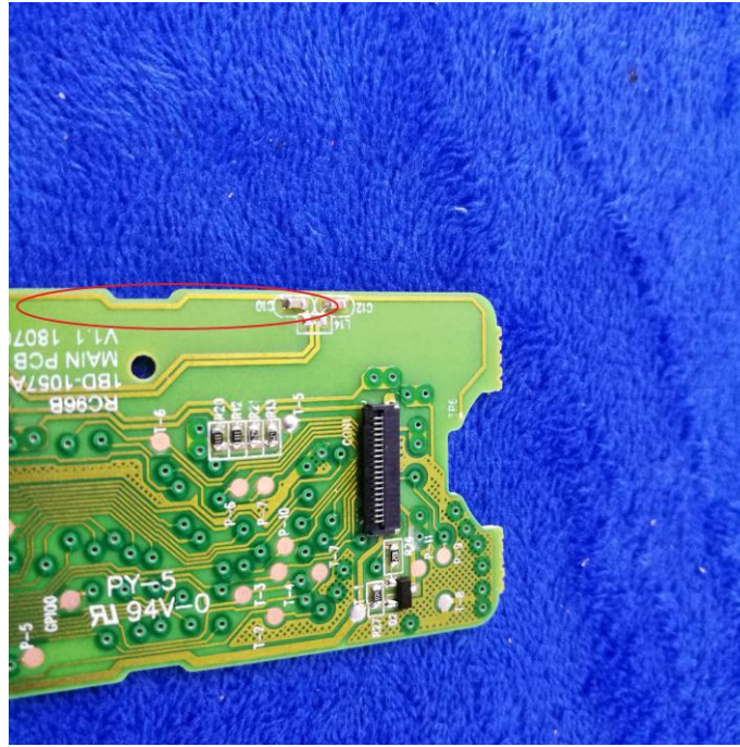
Antenna View 1
