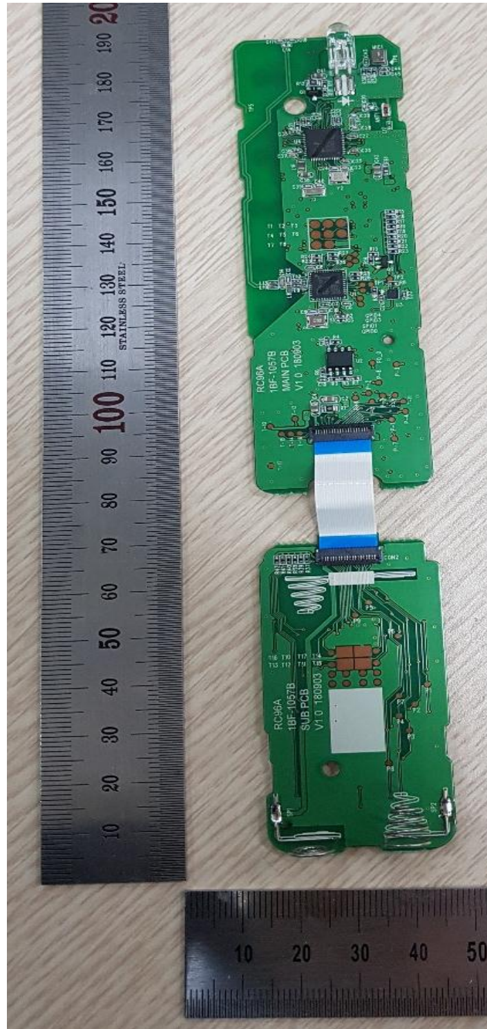
PCB – Front View
