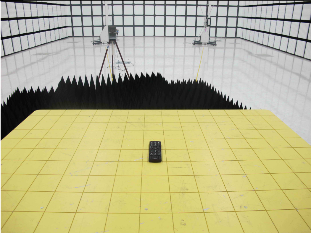
“X” axis
