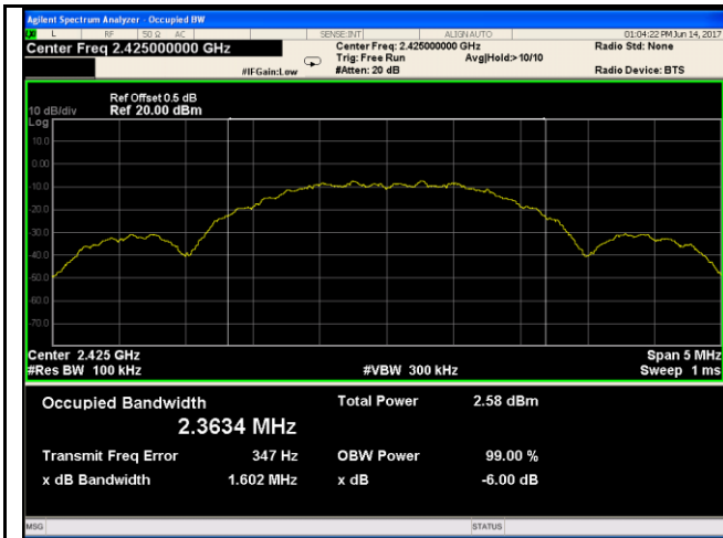
6dB Bandwidth - Low CH 2425
