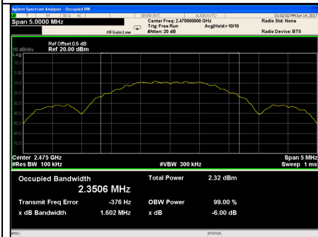
6dB Bandwidth - High CH 2475
