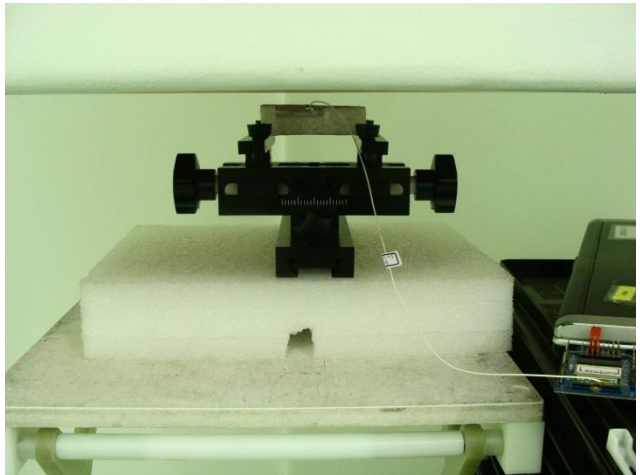
Left Side, Test Separation 0.8 cm
