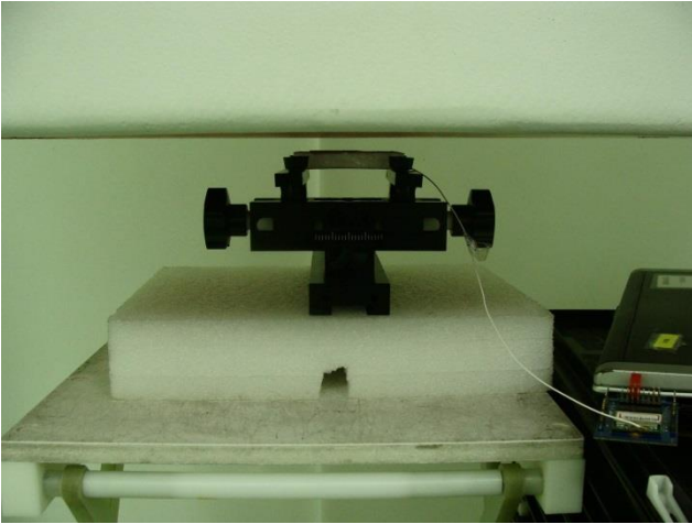
Front, Test Separation 0.8 cm
