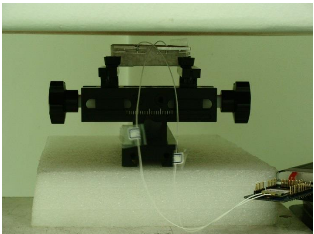
Left Side-2, Test Separation 0.8 cm
