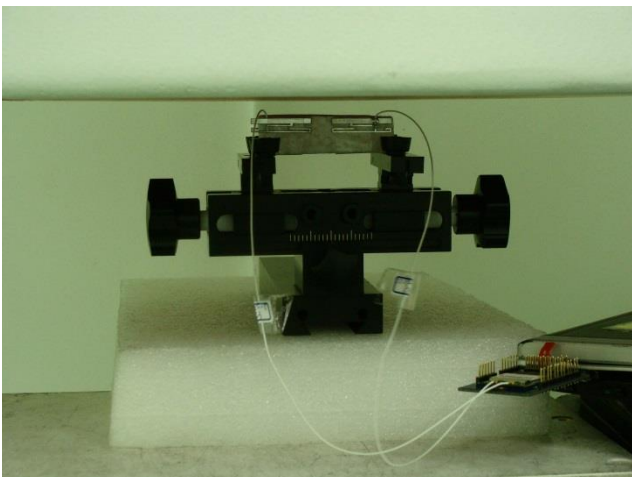
Left Side-1, Test Separation 0.8 cm
