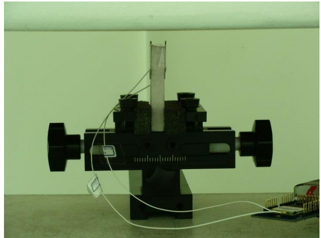
Bottom Side, Test Separation 0.8 cm
