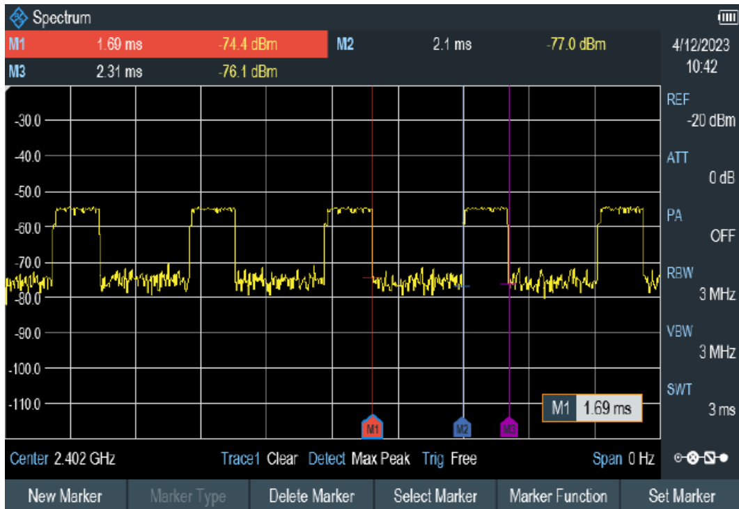
Time-domain plot for Bluetooth transmission signal
