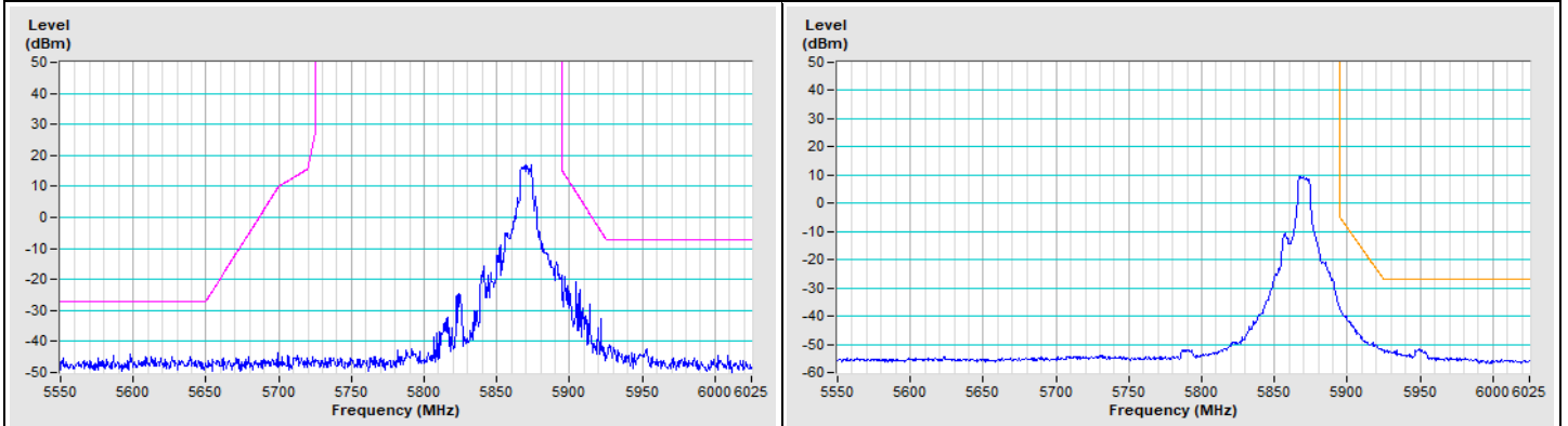
Vertical (Peak)
