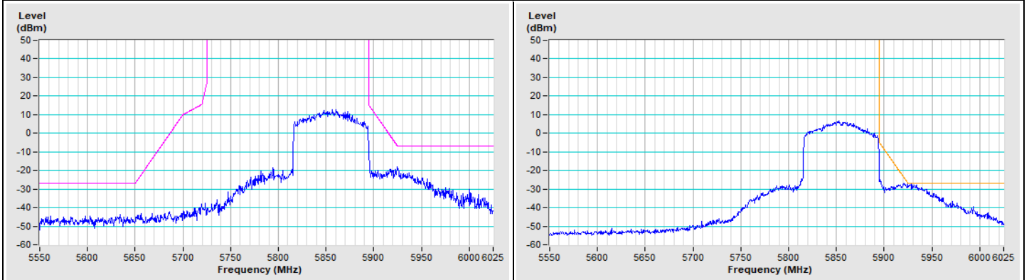
Horizontal (Peak)
