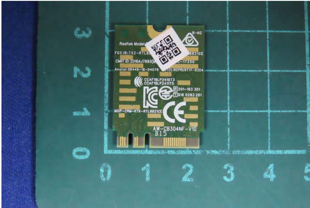
(24) EUT Photo_RTL8821CE
