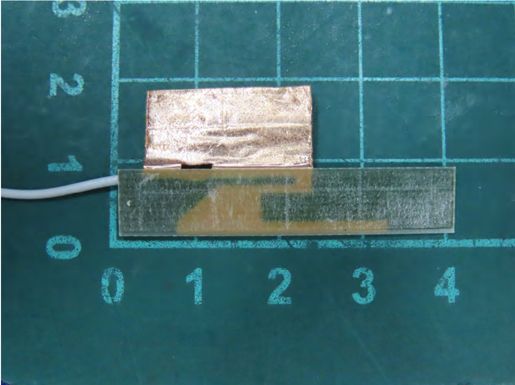
(32) EUT Photo
