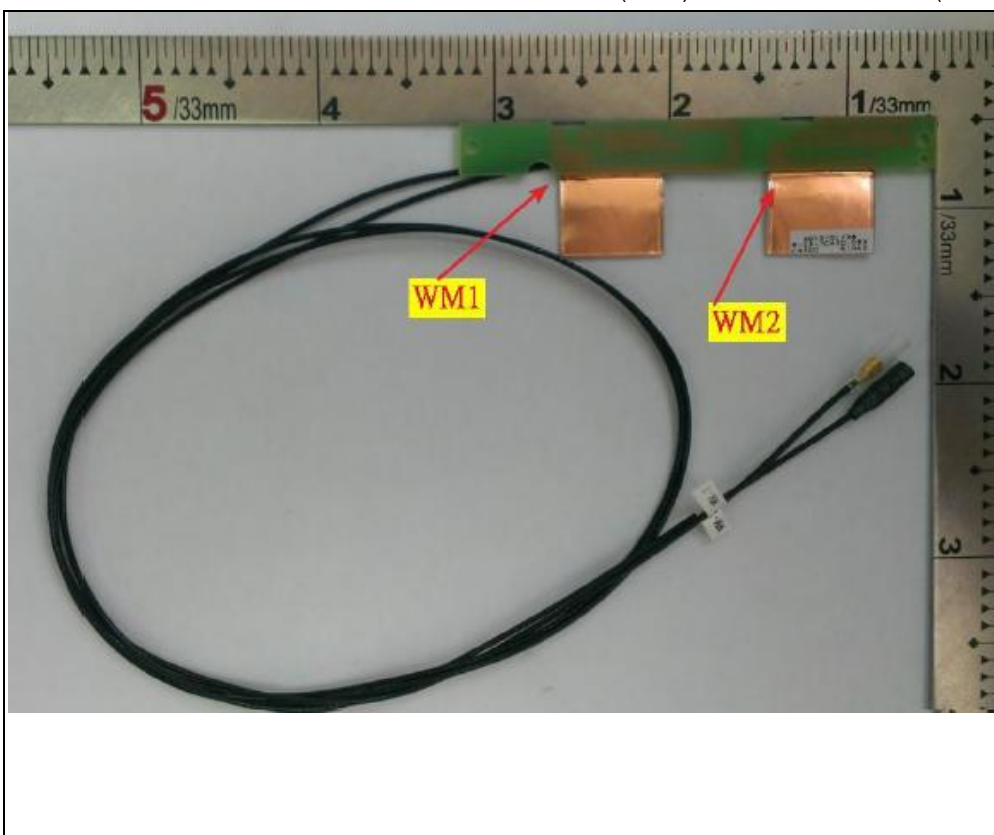
Antenna 33: Brand: WGT / Model: SKC45WMPB03+B (WM1) & SKC45WMPB03+B (WM2)
