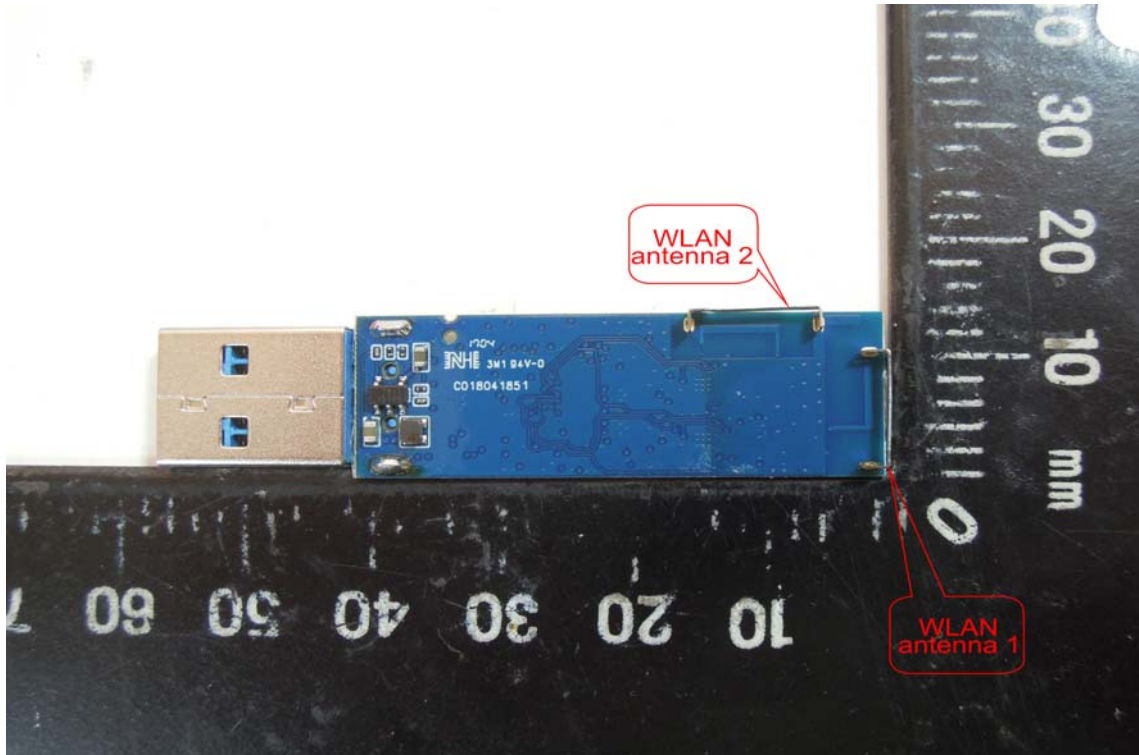
WLAN Antenna
