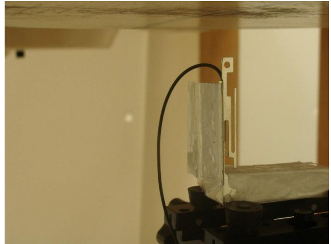
Left Side of the DUT with Phantom 1.7 cm Gap
