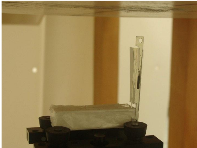
Right Side of the DUT with Phantom 1.7 cm Gap
