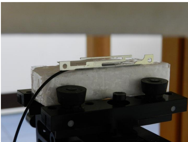
Top Side of the DUT with Phantom 1.7 cm Gap
