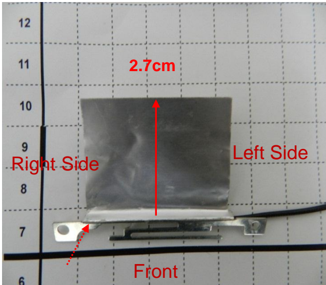
WLAN Antenna <Tx / Rx>
