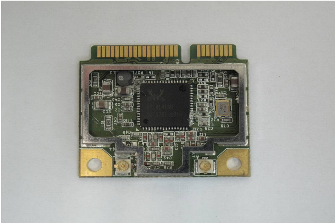
WNC / Main Antenna / Part number: 81.XCC15.G03
