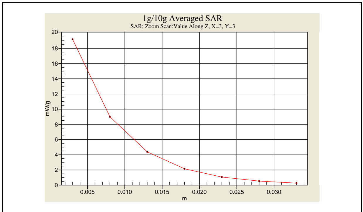
Body-Tissue-Simulating-Liquid 2450MHz
