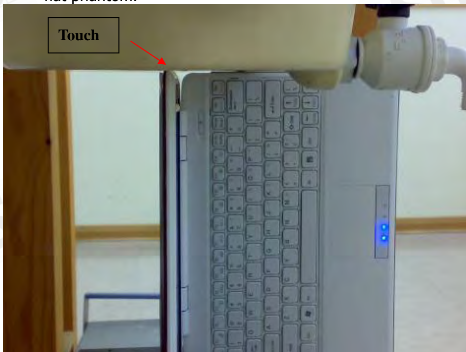
Fig.6 Right side of EUT is paralleled with flat phantom, Right side is contact with flat phantom.
