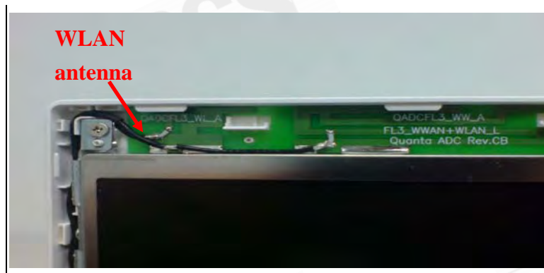
Fig.3 Antenna position of EUT
