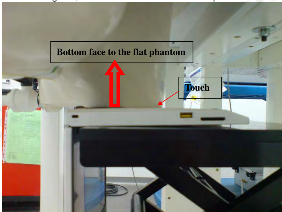
Fig.5 Bottom side of the Netbook is paralleled with flat phantom, open the panel with 90 degrees, bottom side is contact with flat phantom.
