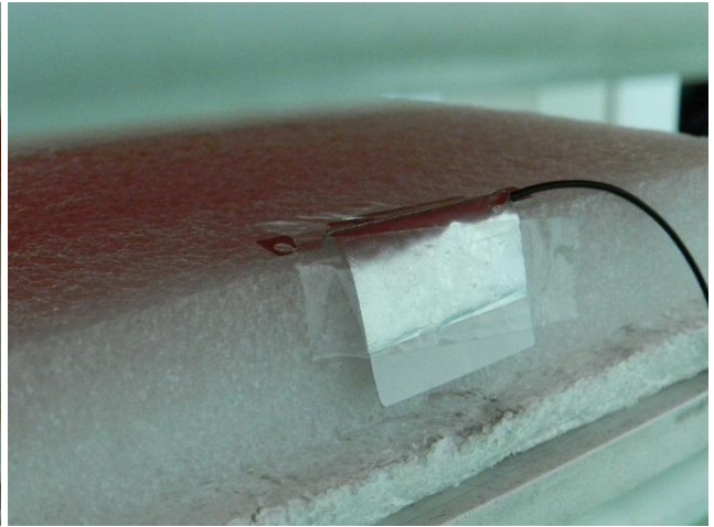
Back of the DUT with Phantom 1.6 cm Gap
