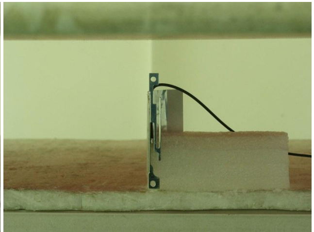
Bottom Side of the DUT with Phantom 1.6 cm Gap
