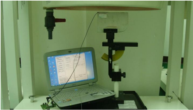
Horizontal Up with Phantom 1.4 cm Gap (Main Antenna Port)
