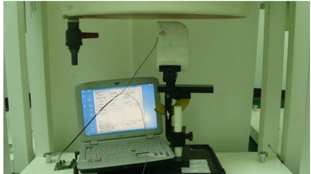
Vertical Up with Phantom 1.4 cm Gap (Main Antenna Port)
