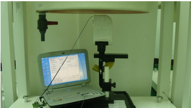
Vertical Down with Phantom 1.4 mm Gap (DUT with Antenna 1)
