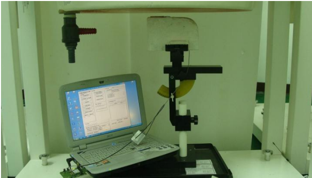
Horizontal Down with Phantom 1.4 mm Gap (DUT with Antenna 2)
