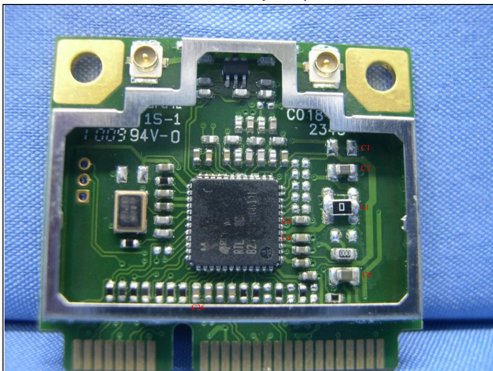
Two antenna connectors <newly sample, PCIe Interface >
