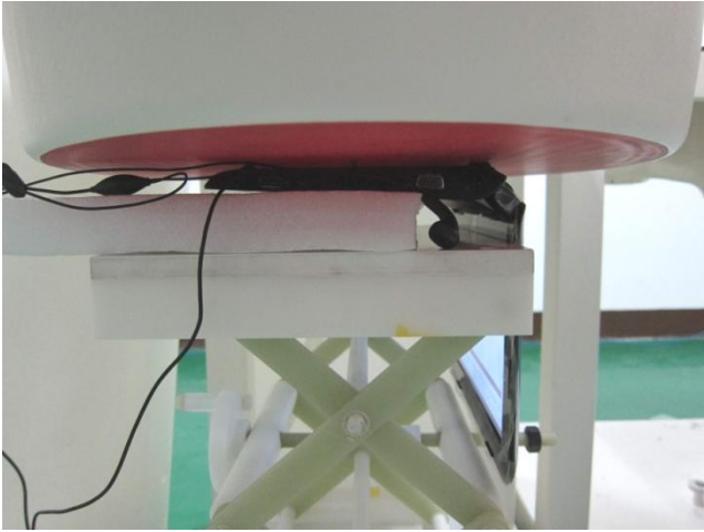
Bottom of the DUT with Phantom 0 cm Gap for (Sample 1)
