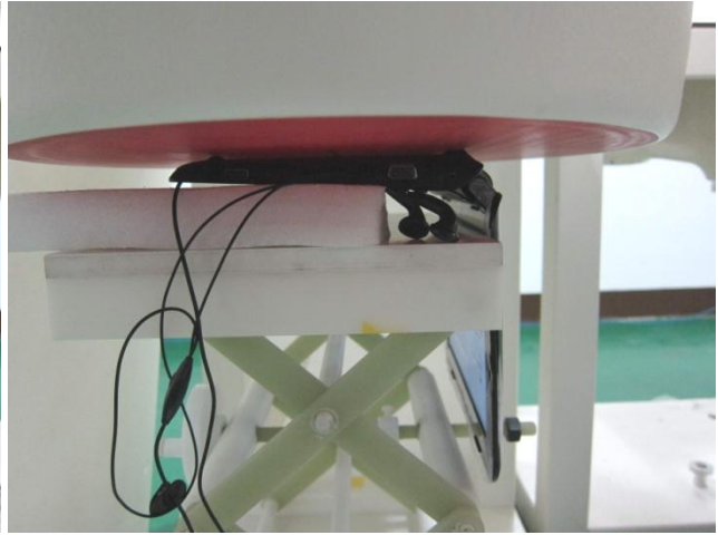
Bottom of the DUT with Phantom 0 cm Gap for (Sample 2)
