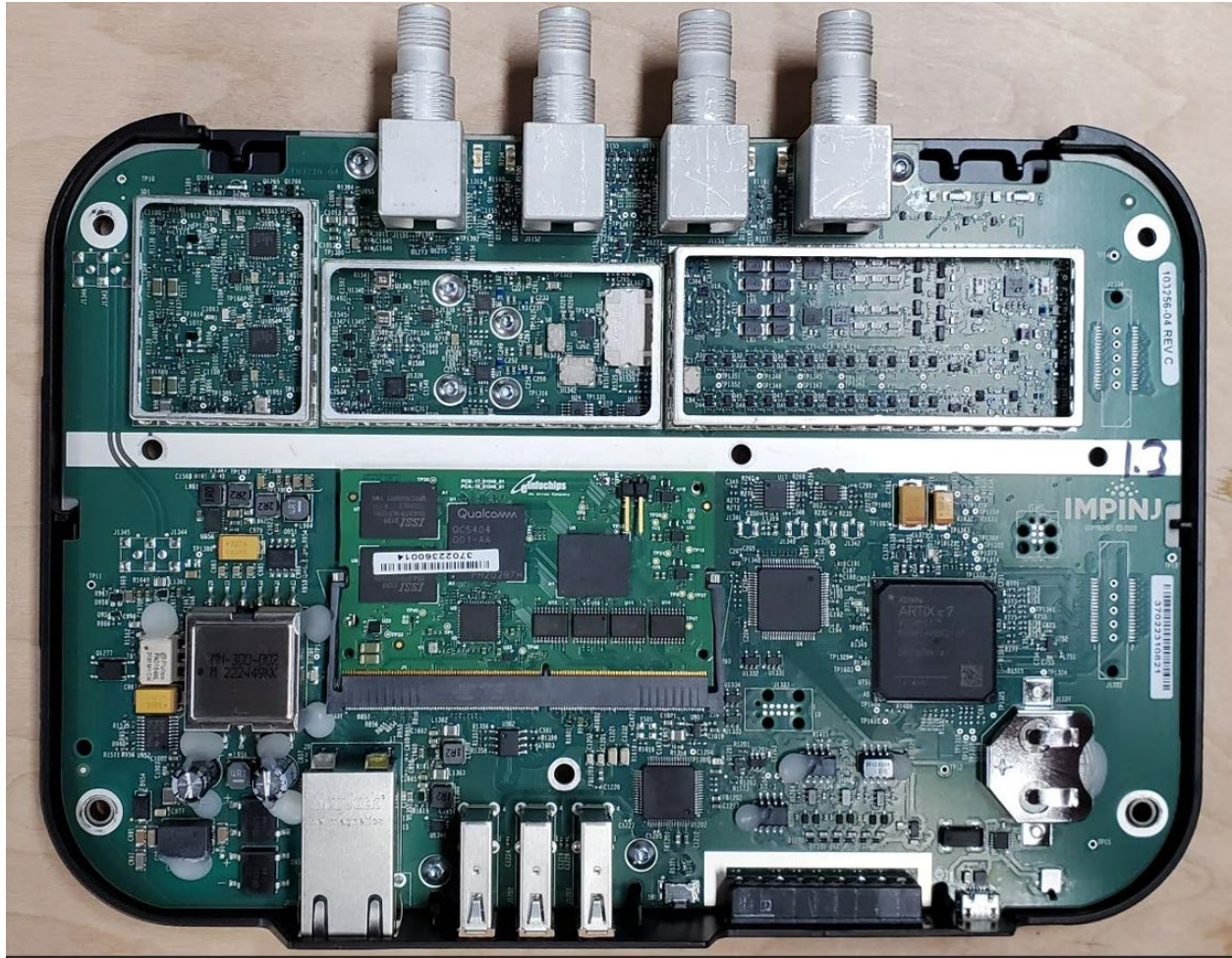
Figure 11: Top Internal View of Reader Components Without Shields
