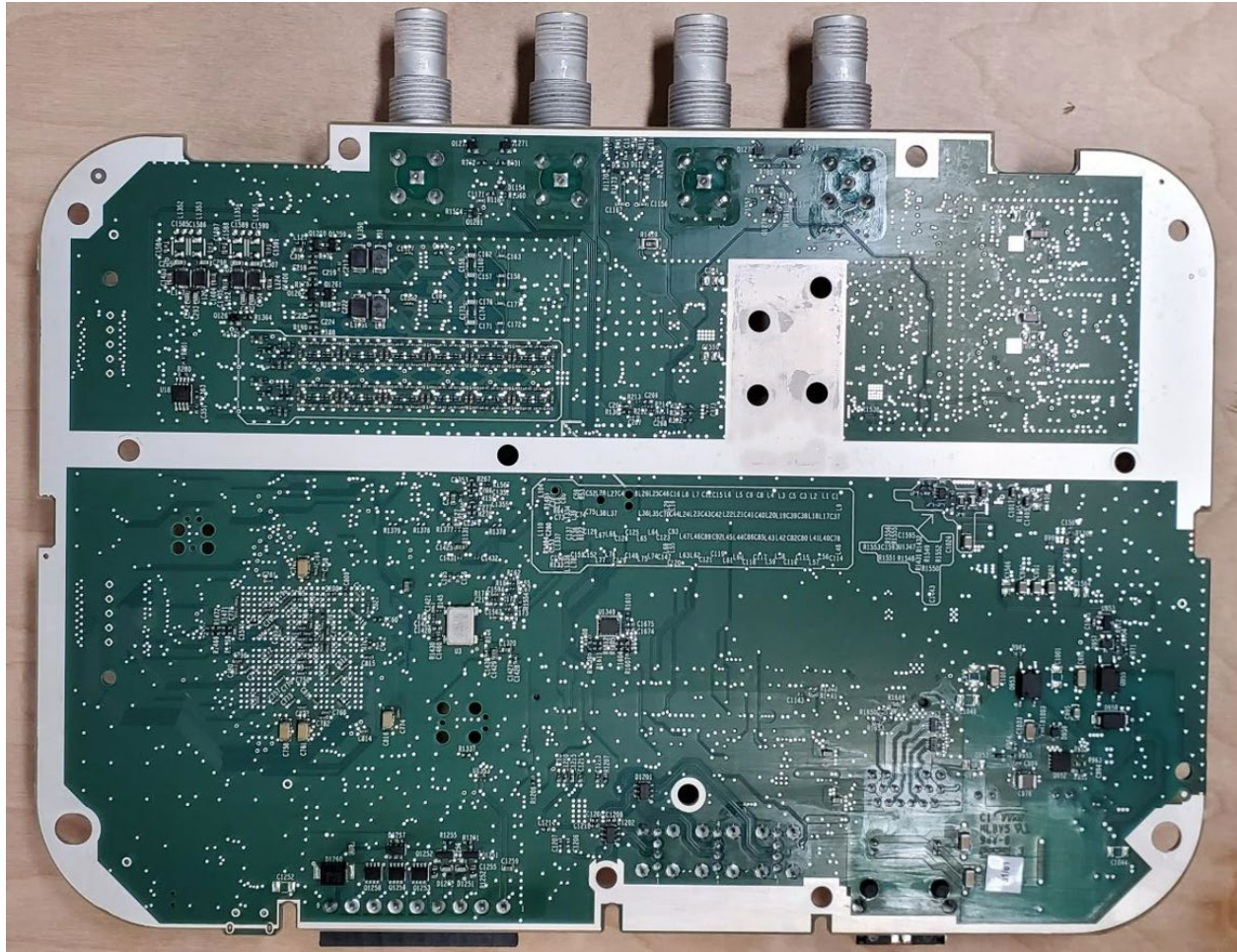
Figure 12: Bottom Internal View of Reader Components
