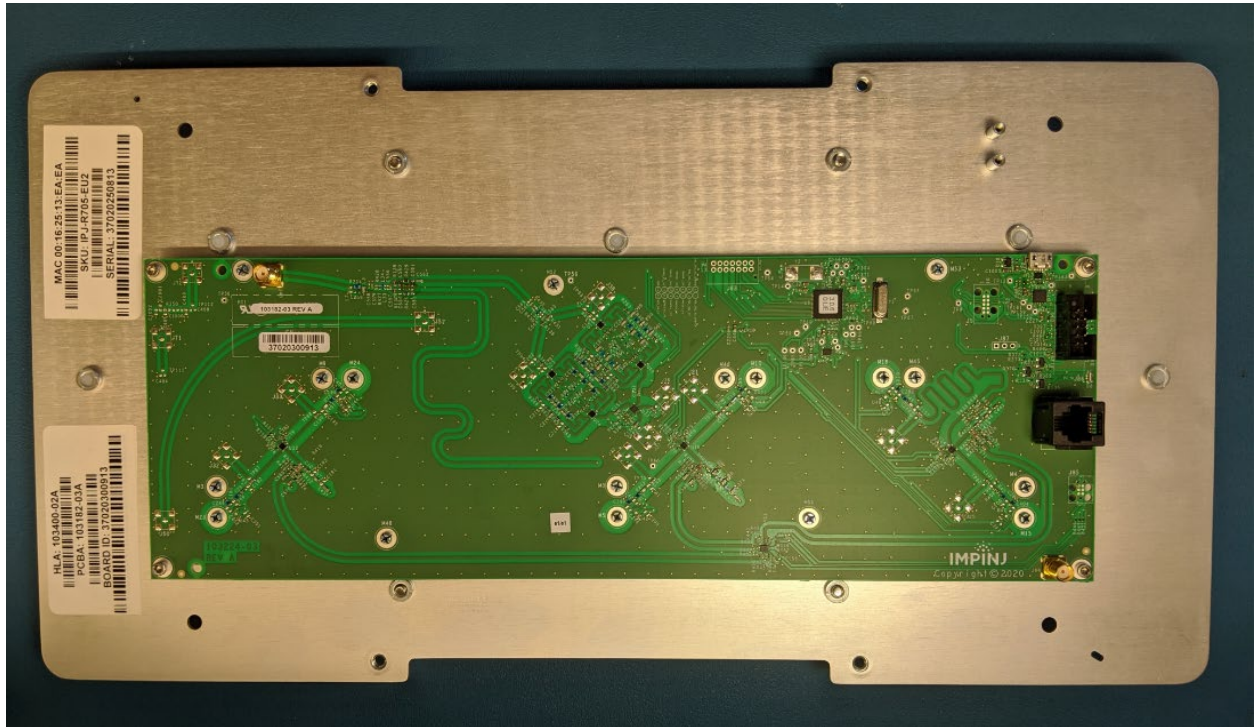
Figure 7: Top Internal View of IPJ-R705 PCBA
