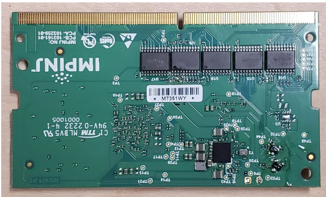
Figure 14: Bottom View of Daughter Card
