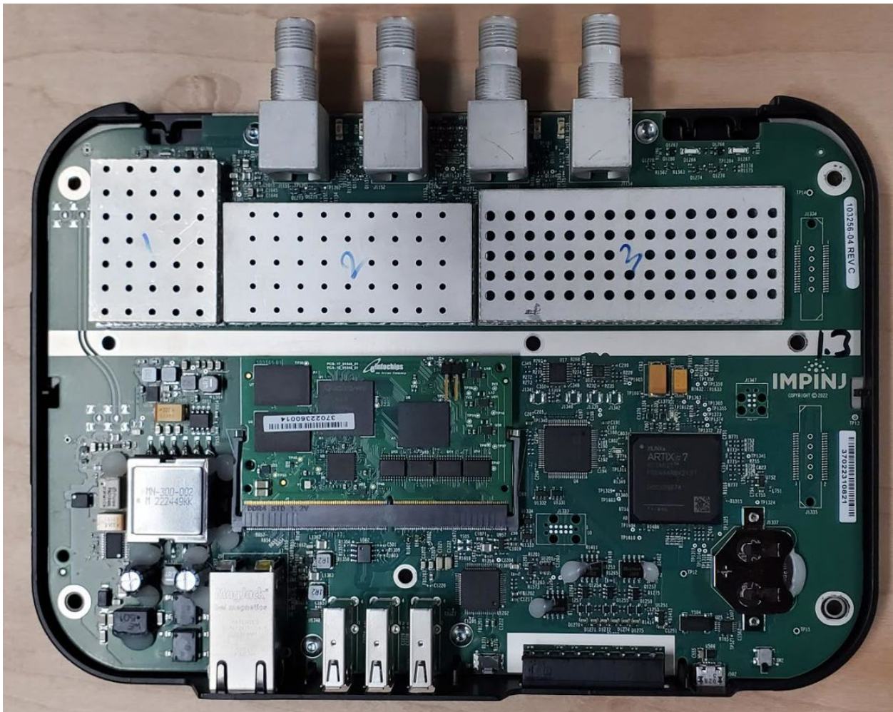
Figure 10: Top Internal View of Reader Components
