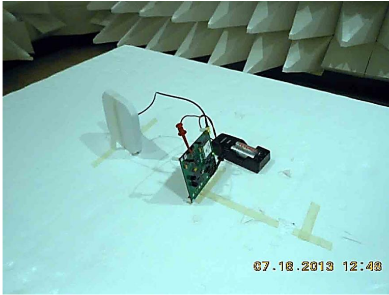
5.5dBi, Z-Axis
