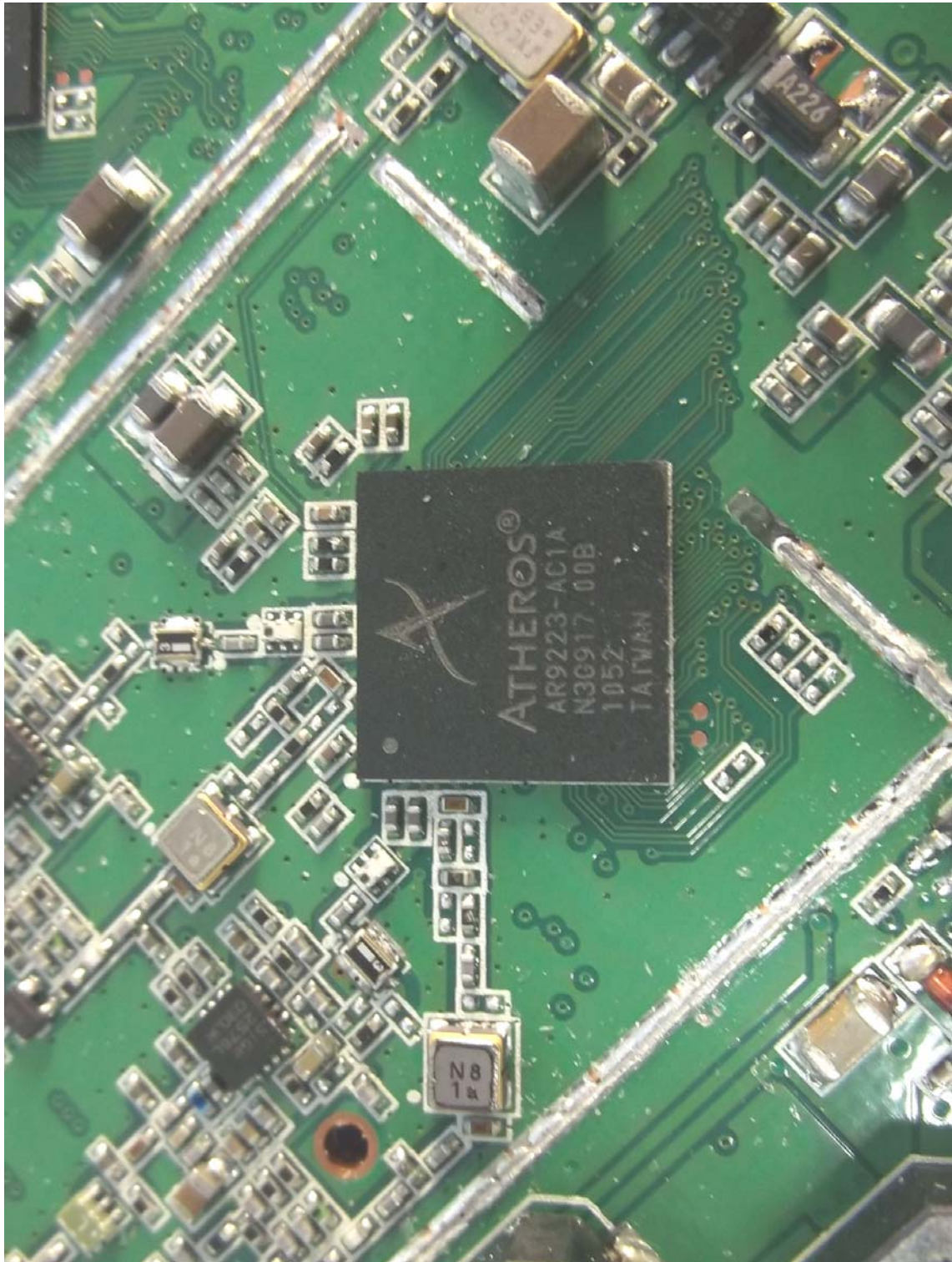
(11) EUT Photo (2.4G_MB)
