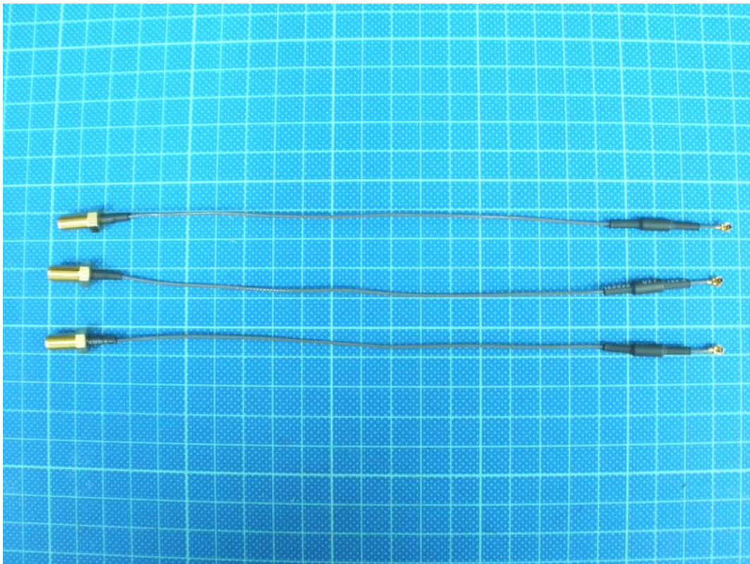
Photo 14: Antenna cable photo of EUT Cable Assy MI-113 L=215MM SMA For I-PEX
