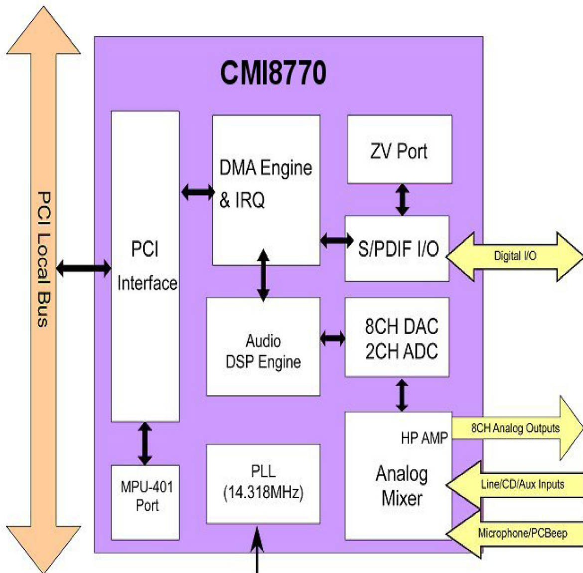
Block Diagram
