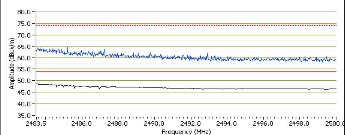
RB 1 MHz; VB 10 Hz (Black trace) Avg; (Blue trace) Pk, Vertical
