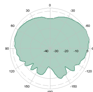
Vertical 5600MHz
