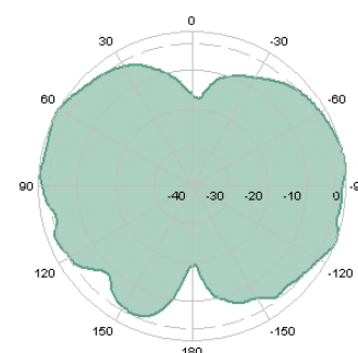
Vertical 2450MHz
