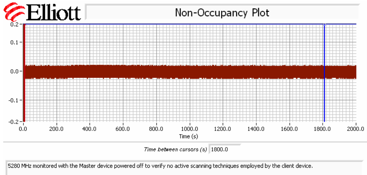
Figure 5 Radar Channel Non-Occupancy Plot (Passive Scan)
