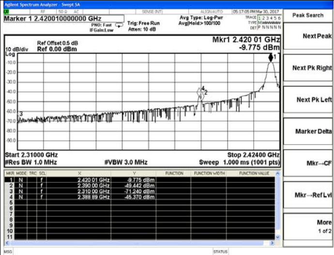
2420 MHz – Peak
