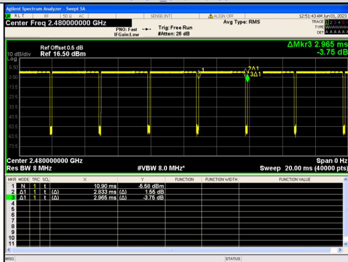
GFSK Channel 78
