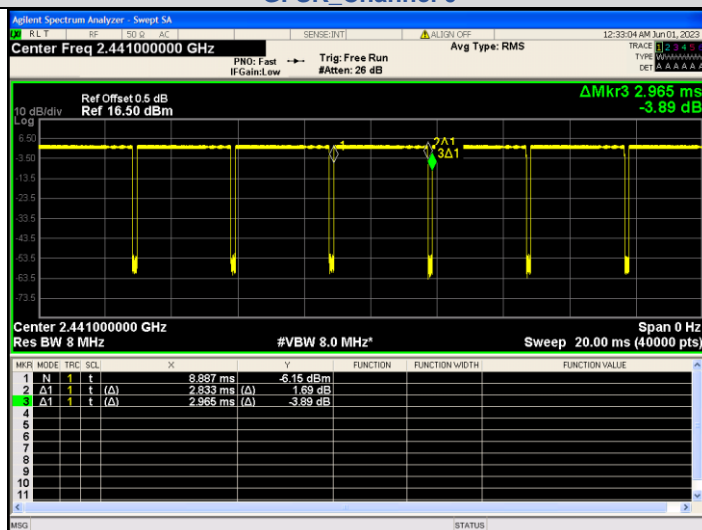
GFSK Channel 39
