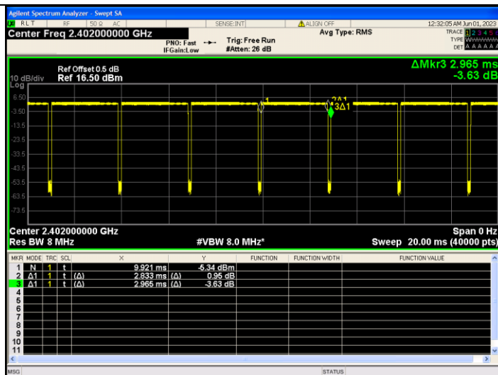
GFSK Channel 0
