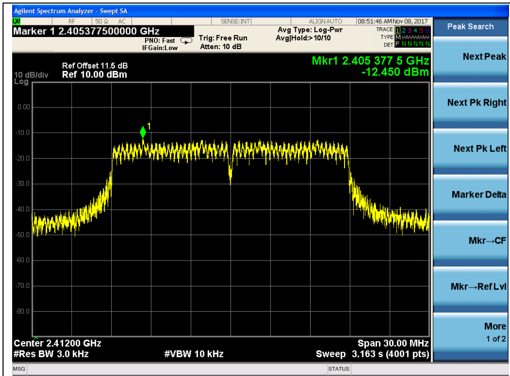
(Channel = 1 @ 802.11n-20MHz)
