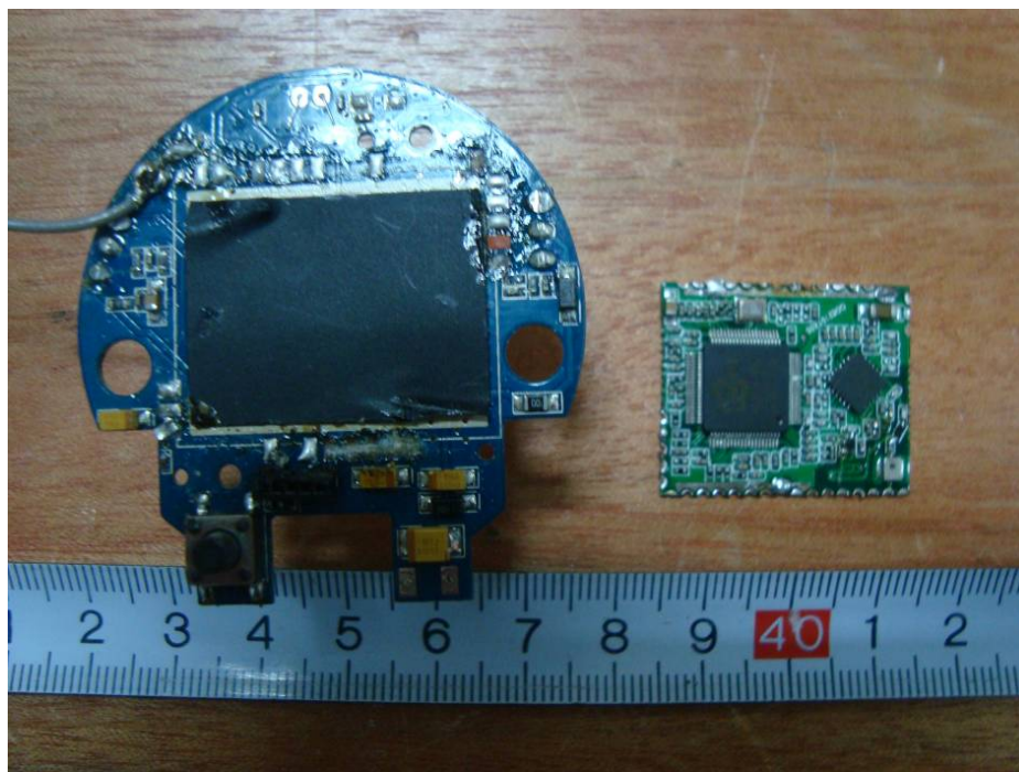
EUT – Camera Board and RF Board View-2
