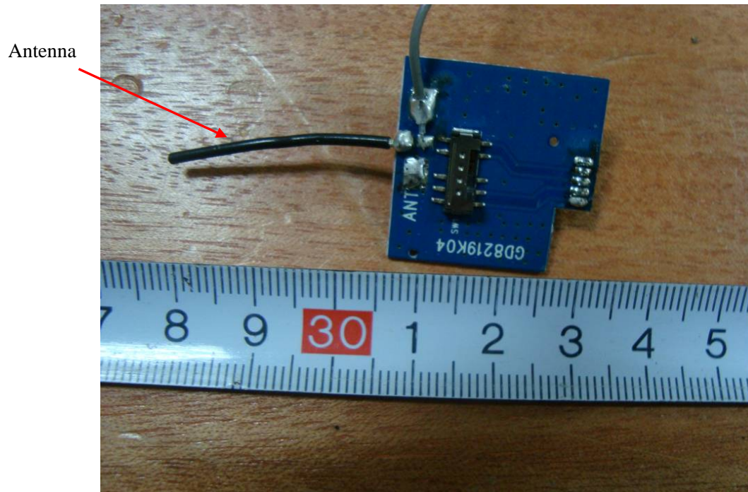
EUT – Antenna Board Bottom View
