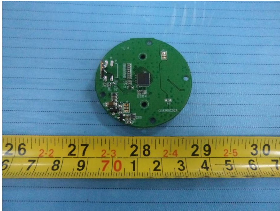
EUT – GD8209C02A Board Bottom View
