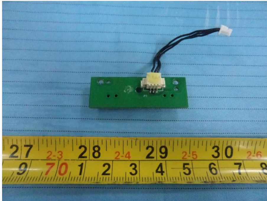
EUT – GD8209K02A Board Top View
