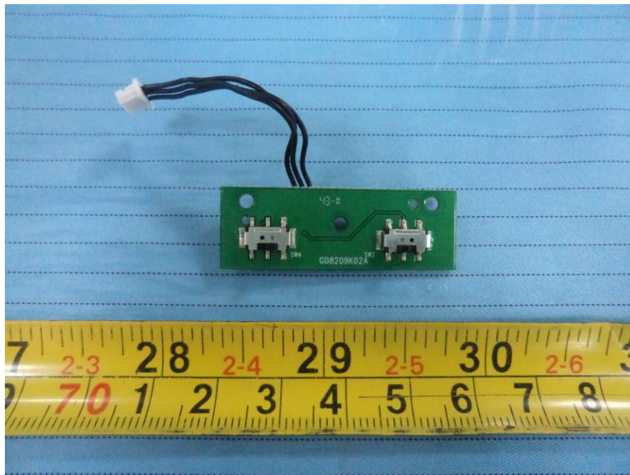
EUT – GD8209K02A Board Bottom View
