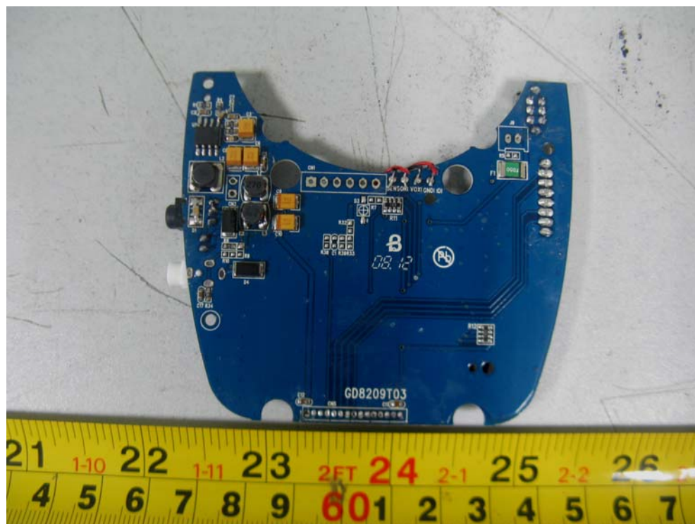
EUT – Power Board Top Components View
