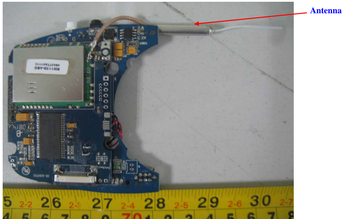
EUT – Power Board Top Components View
