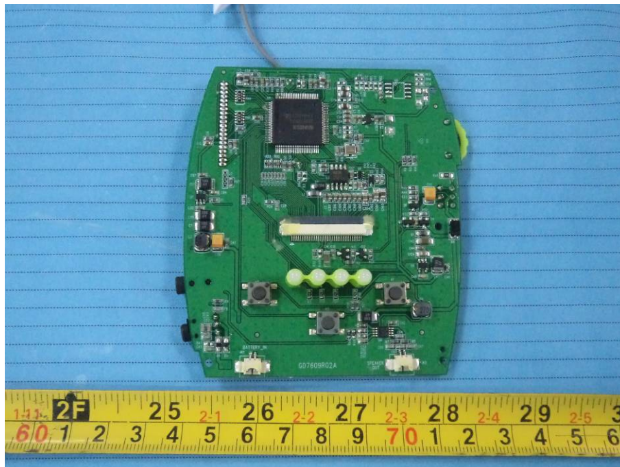
EUT – Main Board without LCD Top View
