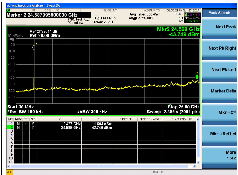
(BPSK Channel = 24, 30MHz to 25GHz)
