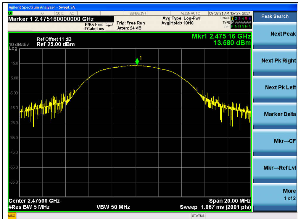
(16QAM, Channel 24, 2475MHz)
