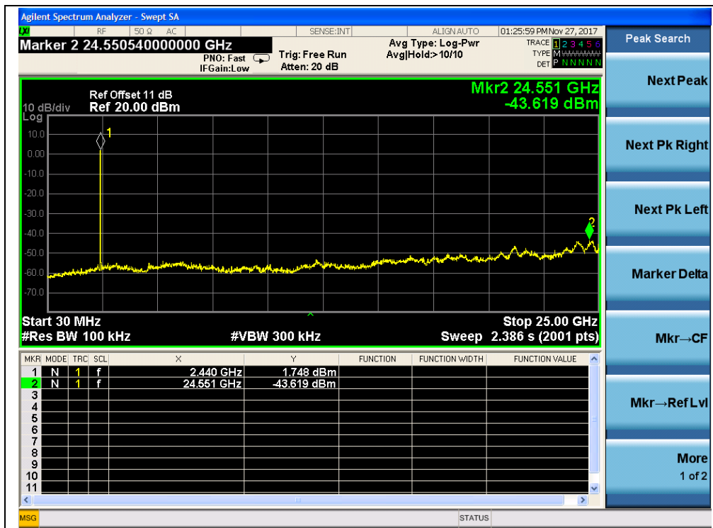
(BPSK, Channel = 13, 30MHz to 25GHz)
