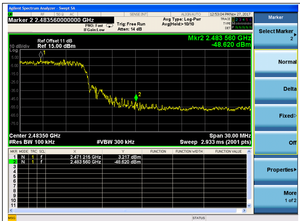
(QPSK, Channel = 24, Band edge with hopping on)
