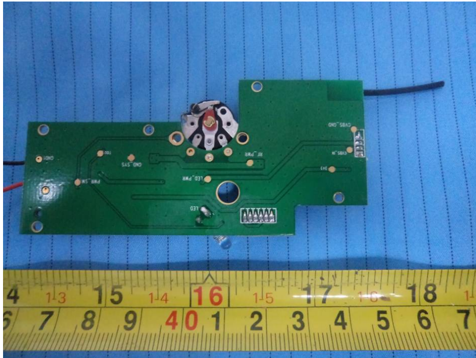
EUT – Connector Board Top View
