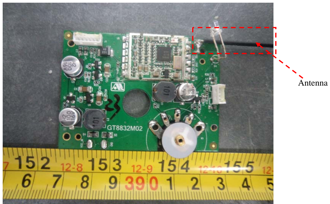
EUT – Main Board Shielding off Components View
