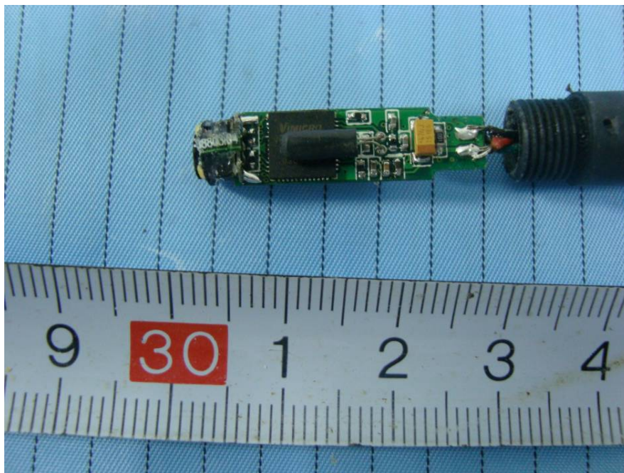
EUT – Camera Board Top View (GB8802)
