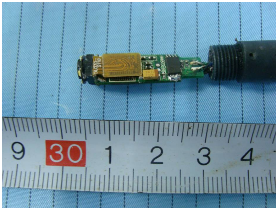
EUT – Camera Board Top View (GB8803)
