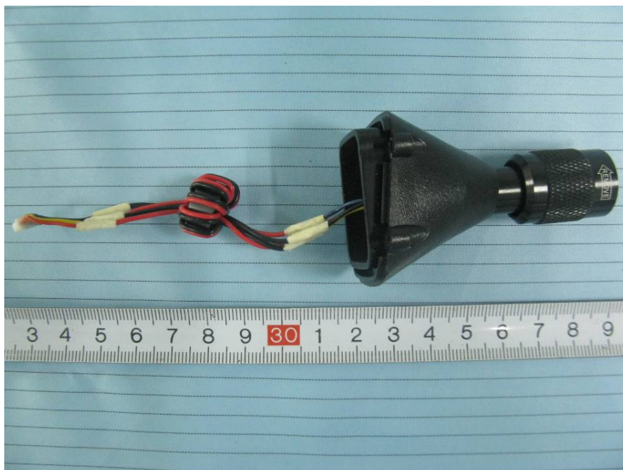
EUT – Connector View (GB8803)
