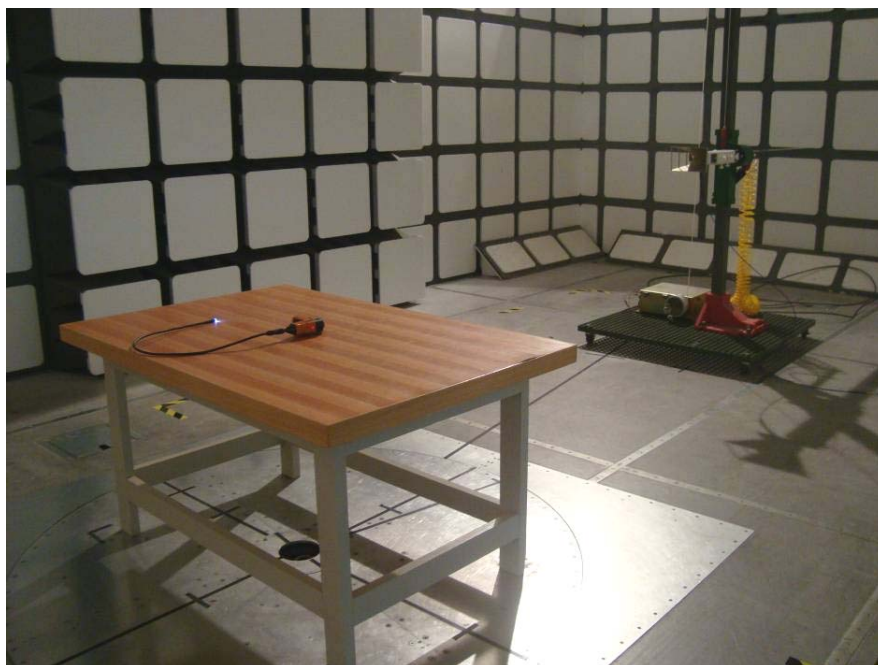
Radiated Emissions - Rear View (Above 1 GHz, GB8803)
