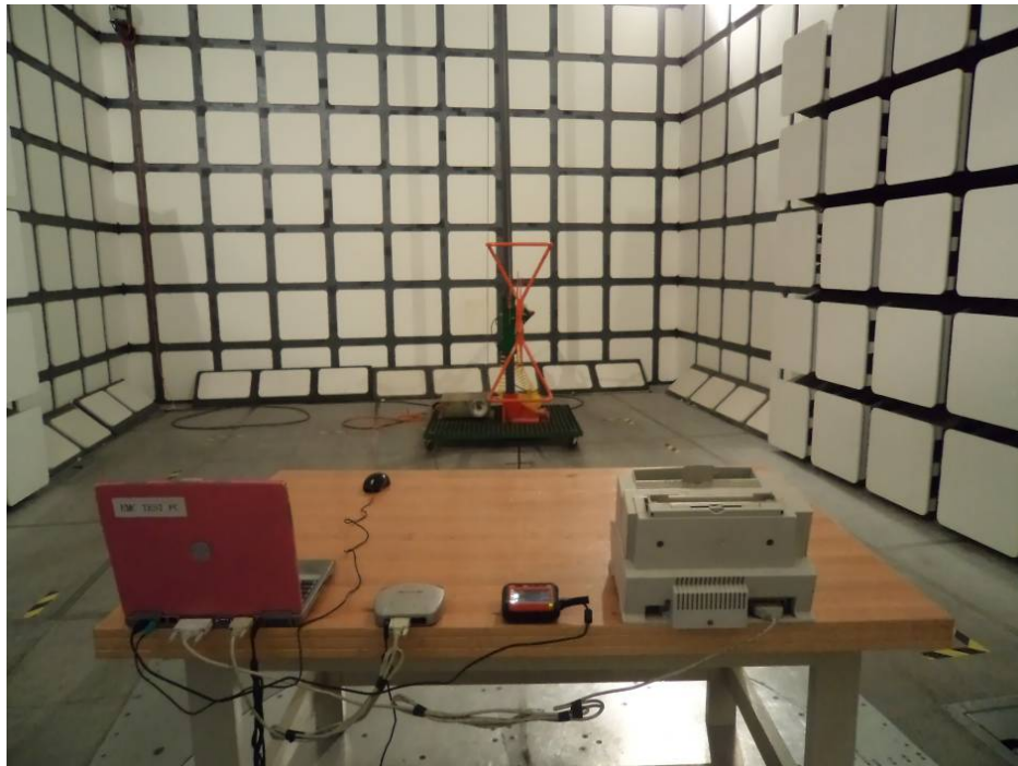
Radiated Emissions for Test Mode 3 - Rear View
