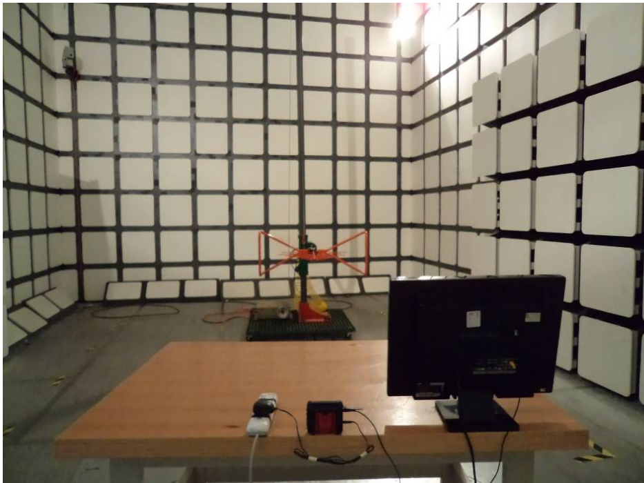
Radiated Emissions for Test Mode 1 - Rear View
