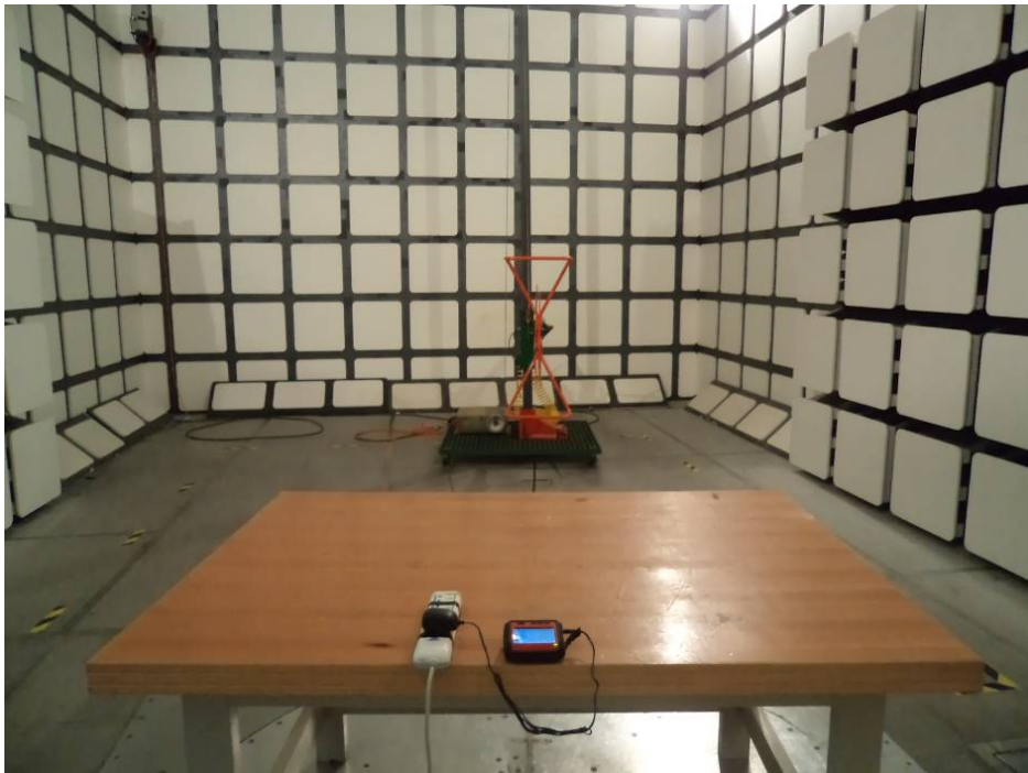
Radiated Emissions for Test Mode 2 - Rear View
