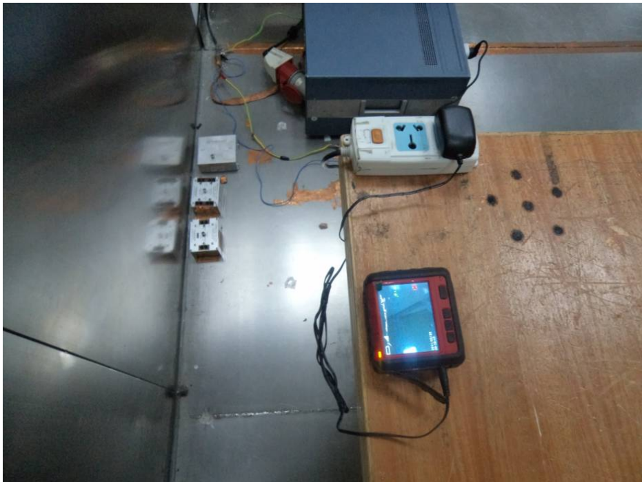
Conducted Emissions for Test Mode 2 - Side View
