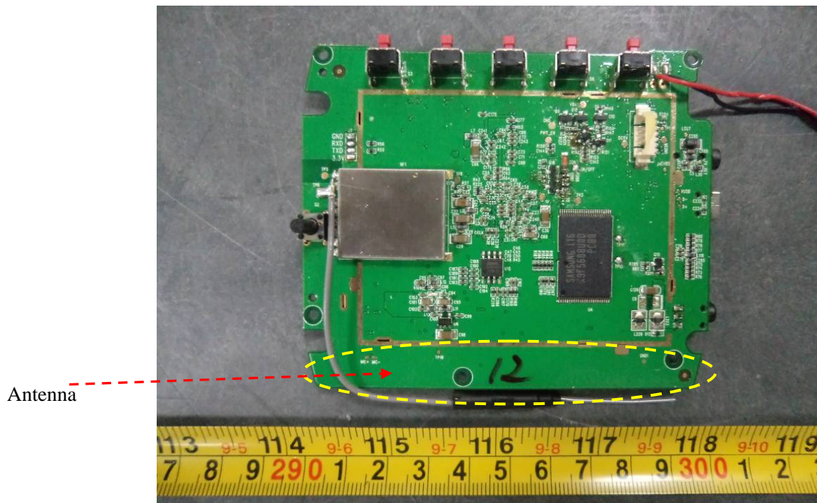
EUT – Main Board Shielding off Bottom View
