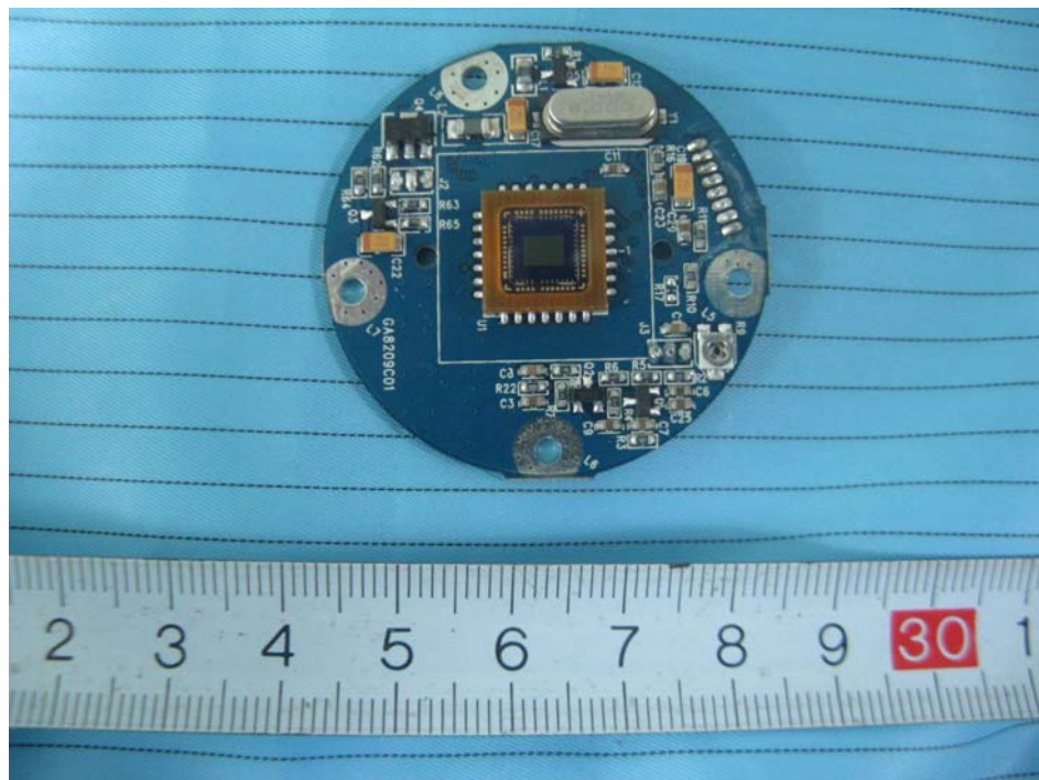
EUT – Video Board Top View
