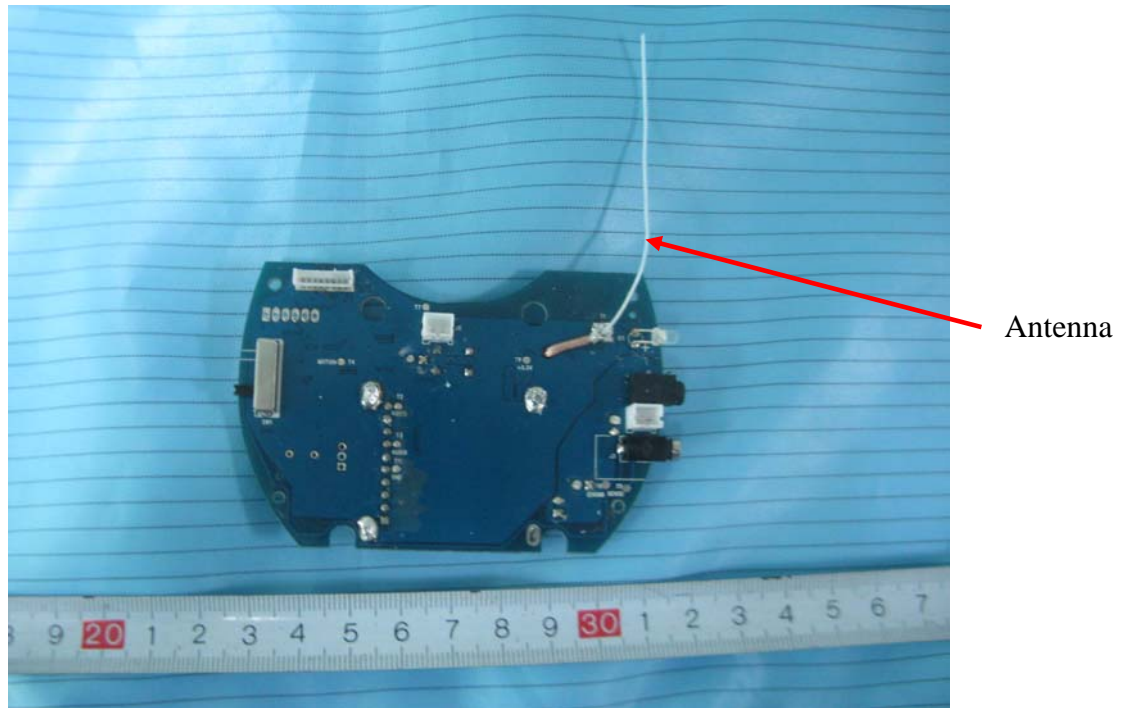
EUT – Video Board Top View
