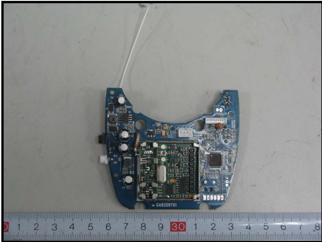
EUT-Main Board Components View
