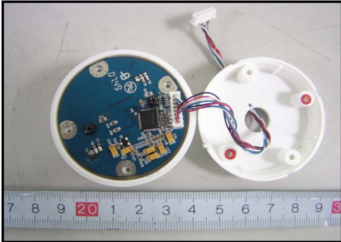
EUT-Camera Board Components View
