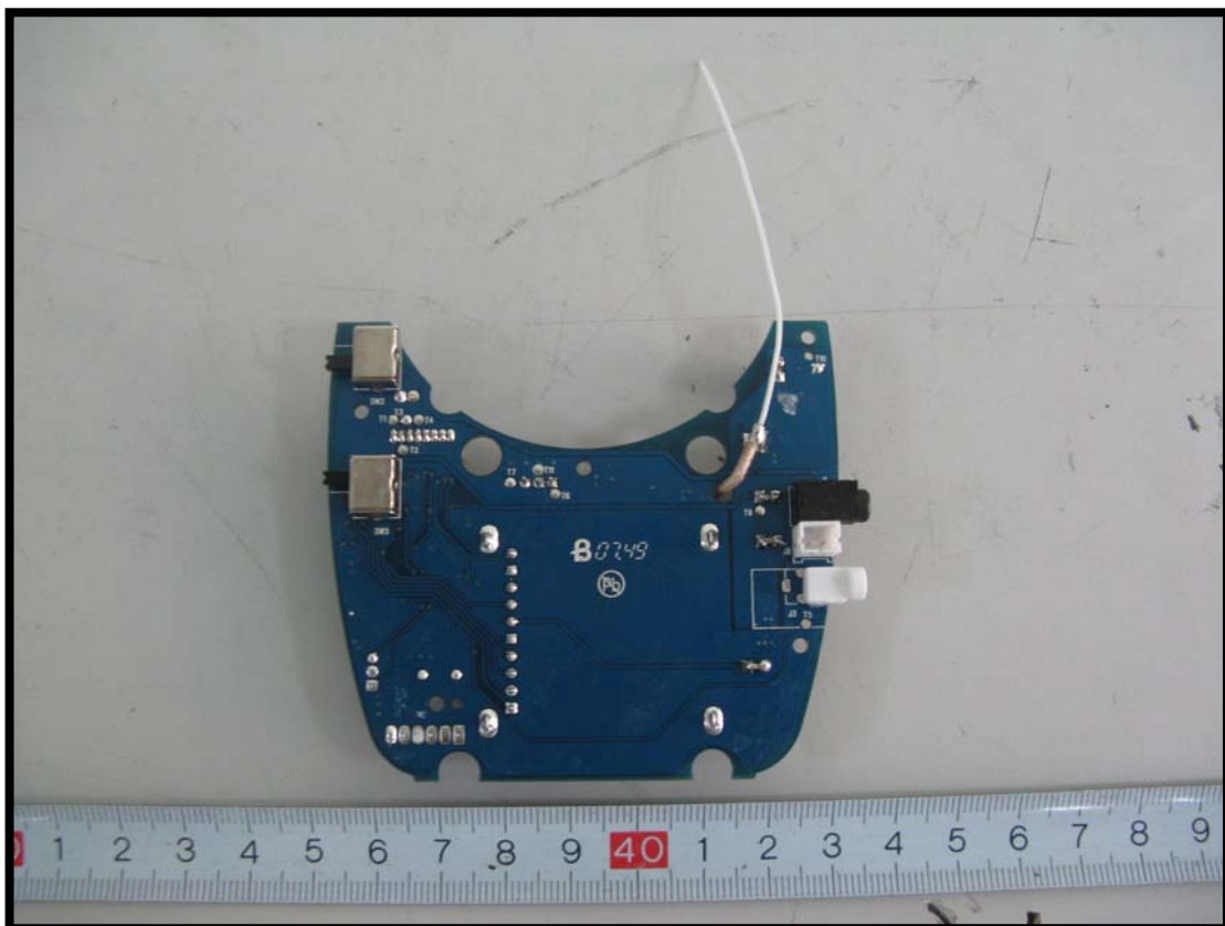
EUT-Main Board Circuits View
