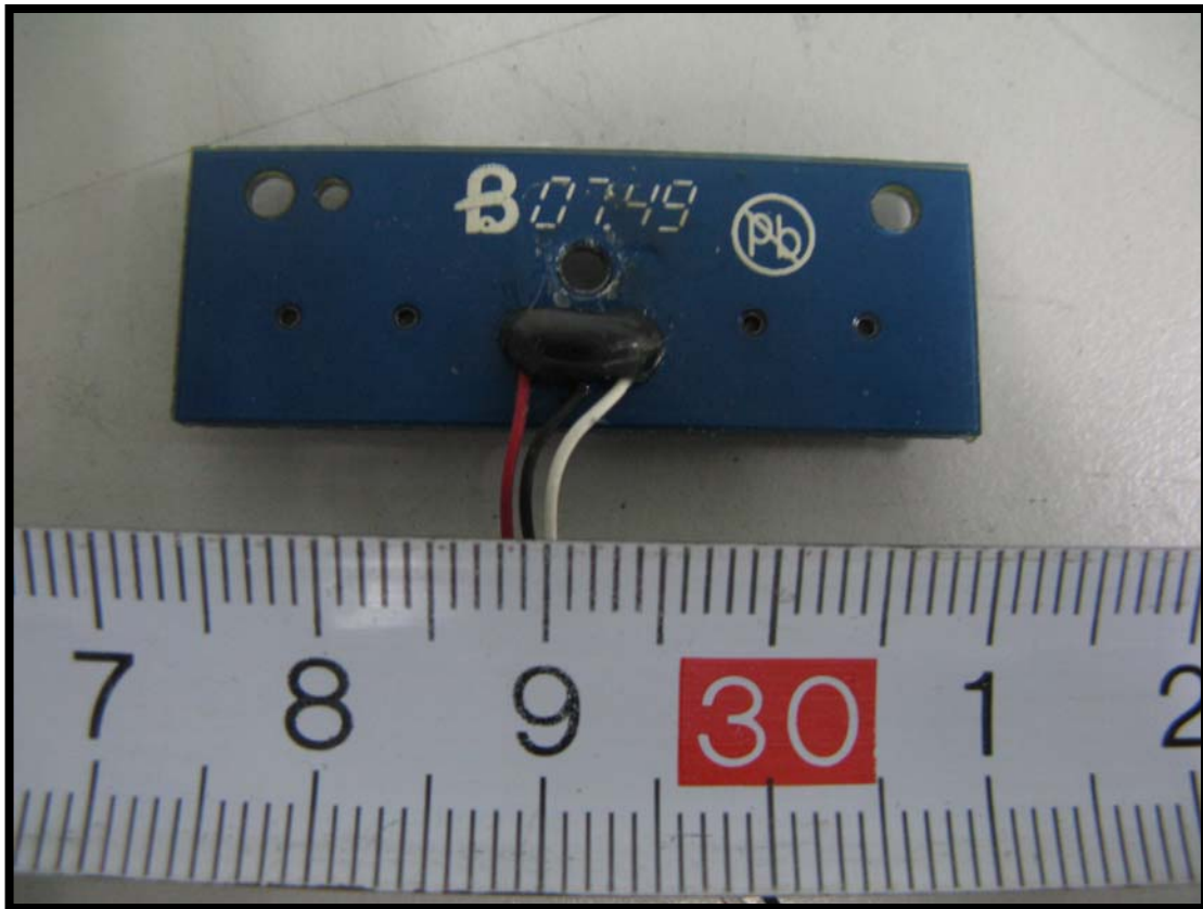
EUT-Control Board Circuits View
