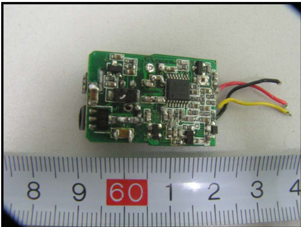
EUT –Main Board without Antenna Top View
