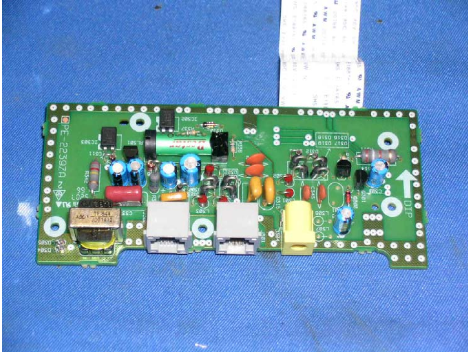
Base Unit Telephone Line Jack and AC Jack comp side
