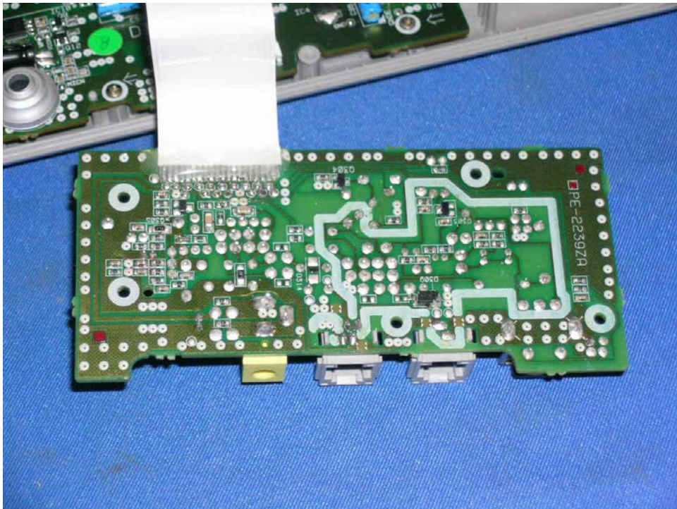
Base Unit Telephone Line Jack and AC Jack solder side
