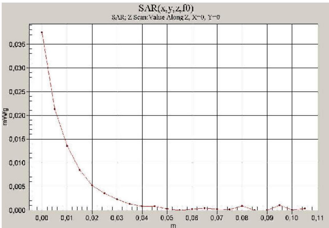
Z-axis scans 1900 MHz body
