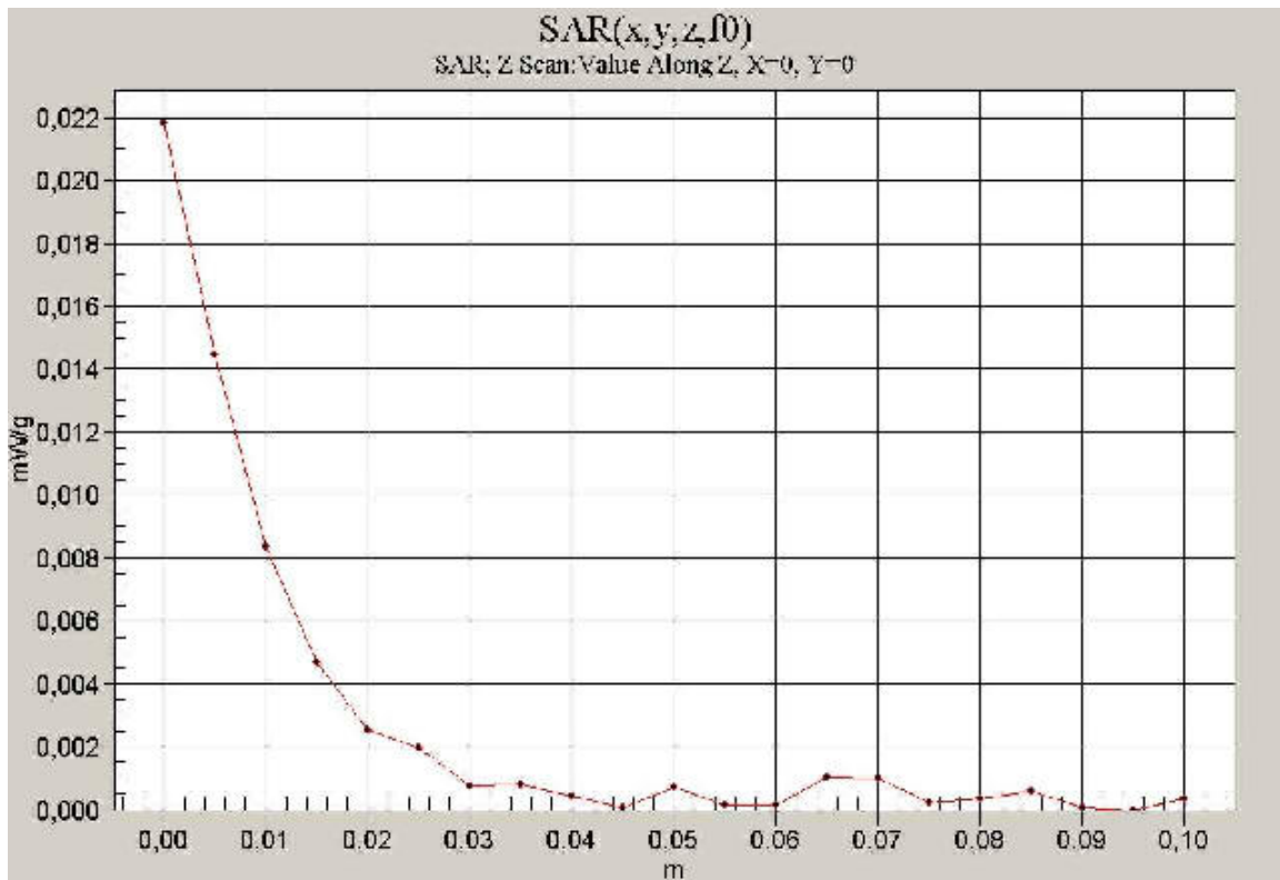
Z-axis scans 1900 MHz head
