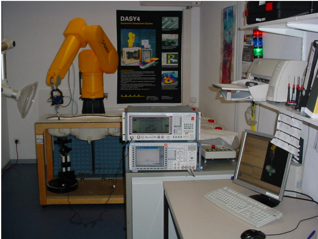
Photo 2: UPCS System
